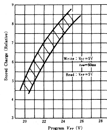
Fig. 4 Typical Programming Characteristics of EPROMs.
