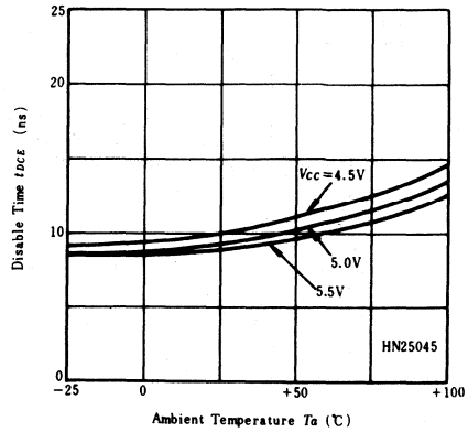
DISABLE TIME vs. AMBIENT TEMPERATURE (HN25045)
