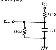
Load Circuit (B)
