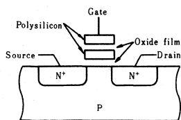
Fig. 2 Cross section of memory transistor
