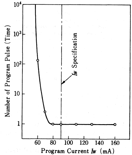
Fig. 11 Program Pulse - I_w Characteristic of S Series (HN25169S)
