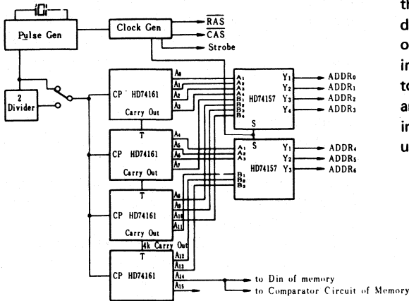
Fig. 2 Marching Pattern Generating Circuit
