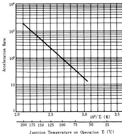
Fig. 2 Example of derating of ECL
