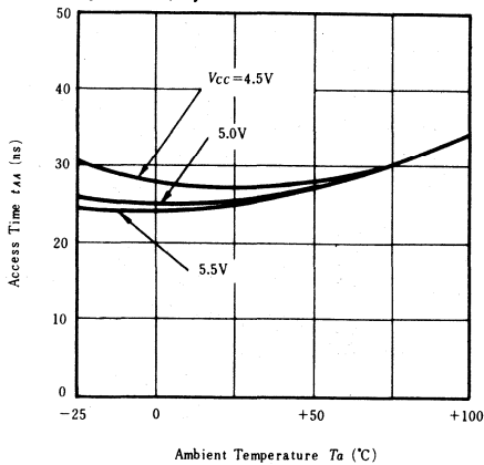
ACCESS TIME vs. AMBIENT TEMPERATURE (HN25044)
