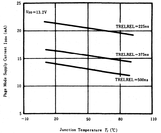
IDD4 (PAGE-MODE CYCLE) vs. T_j
