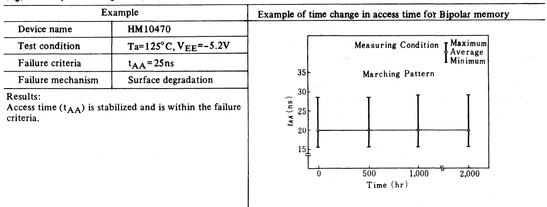
Fig. 1 Example of Change in Bipolar Memory Characteristics
