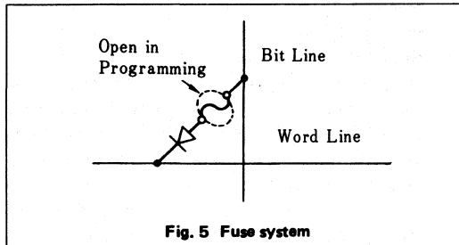
Fig. 5 Fuse system
