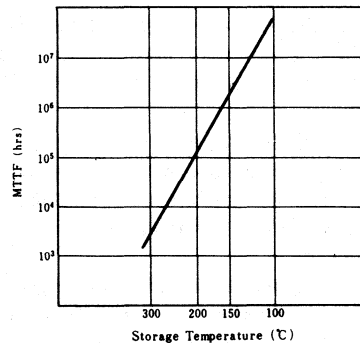
Fig. 6 Typical Data Retention Characteristics
