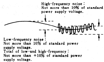
Fig. 5 Power source noise
