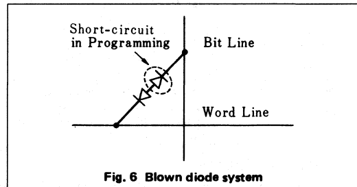
Fig. 6 Blown diode system
