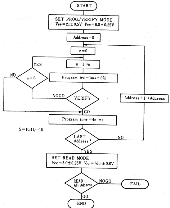
High Performance Programming Flowchart
