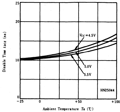
DISABLE TIME vs. AMBIENT TEMPERATURE (HN25044)
