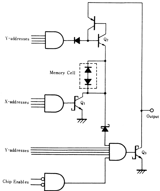
INTERNAL PROGRAMMING CIRCUIT
