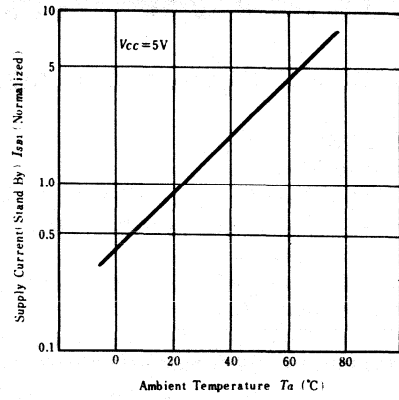
SUPPLY CURRENT vs. T_a (STANDBY)
