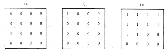
Fig. 1 Addressing method for 16 bits memory in the Marching pattern
