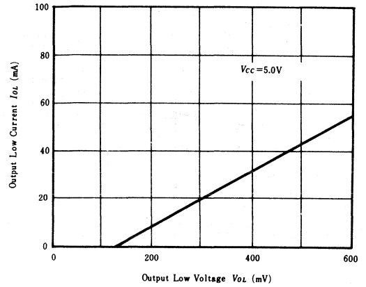
OUTPUT LOW CURRENT vs. OUTPUT LOW VOLTAGE
