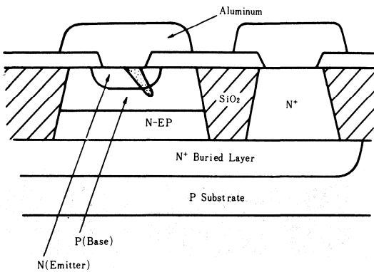
PROGRAMMED CELL (CROSS SECTION)
