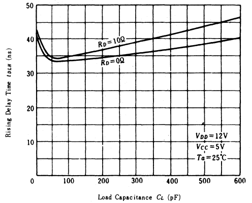
RISING DELAY TIME vs. LOAD CAPACITANCE (2)
