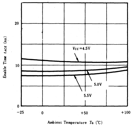
ENABLE TIME vs. AMBIENT TEMPERATURE (HN25045)
