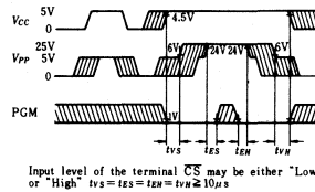
Fig. 1. Power on-off timing sequence.
