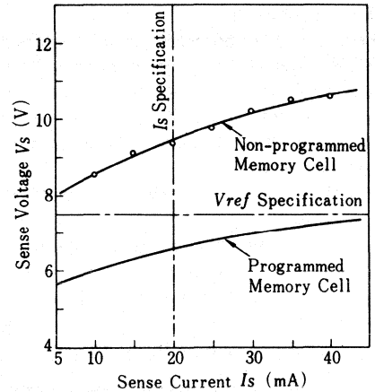
Fig. 9 V_s - I_s Characteristic of S Series (HN25169S)
