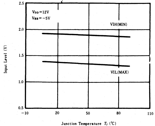
ADDRESS AND DATA INPUT LEVELS vs. T_j
